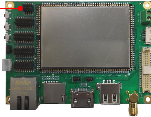
J40: Front panel audio 10-pin header (Pitch 1.27mm x 2.54mm)
